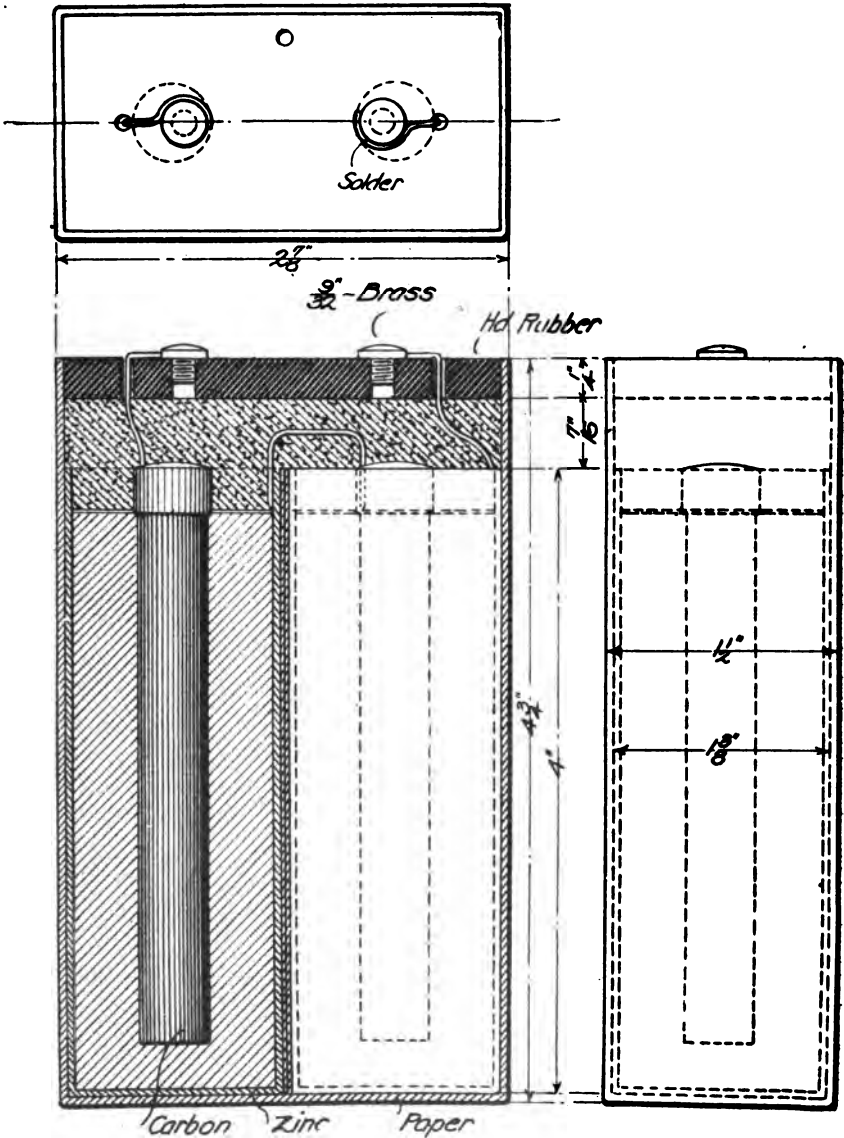
FIG. 5.—Cavalry buzzer dry cell.
